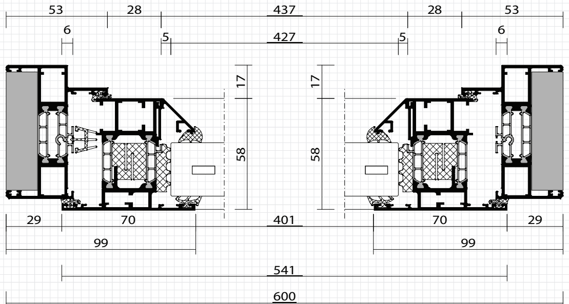
Top Cross Section
